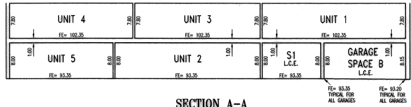
SECTION A-A 929 BUILDING
